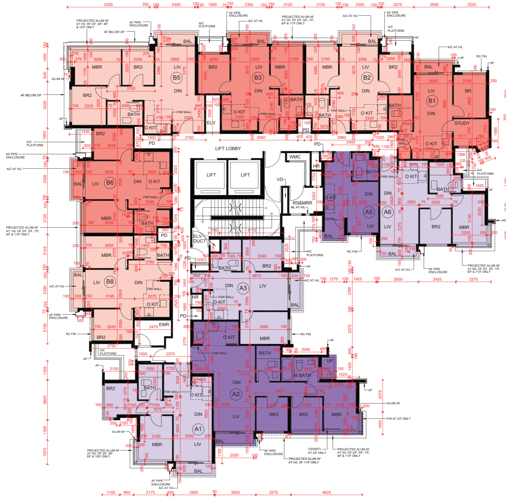
GREENWOOD TOWER 5 2/F-3/F AND 5/F-11/F FLOOR PLAN
